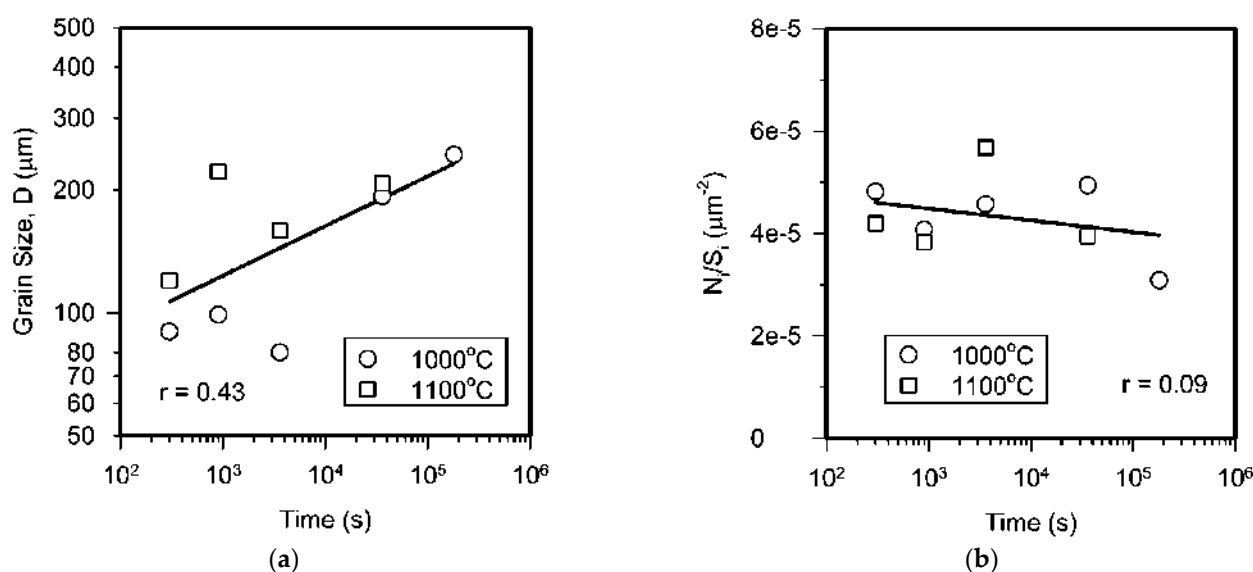
Figure 5. Effect of annealing time on the grain size (a) and the number of grain boundary interruptions per unite area (b) for a 316L stainless steel subjected to recrystallization annealing followed by grain growth. The values of the determination coefficient ( r ) correspond to the linear regressions.
