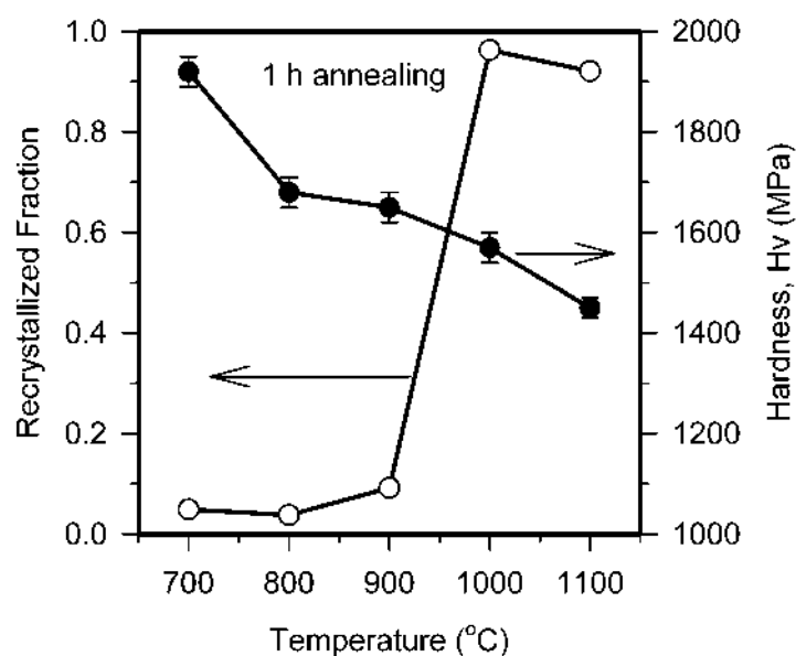
Figure 2. Recrystallized fraction calculated as the area fraction of grains with grain orientation spread below 1^\circ and the hardness of the steel samples subjected to 5% cold rolling reduction followed by 1 h of annealing.
