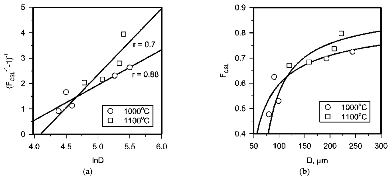
Figure 7. Change in the \Sigma^{3n} CSL boundary fraction ( F_{\text{CSL}} ) with increasing the grain size ( D ) shown as plots of (F_{\text{CSL}}^{-1} - 1)^{-1} vs. \ln D (a) and F_{\text{CSL}} vs. D (b) in a 316L stainless steel subjected to recrystallization annealing followed by grain growth.
