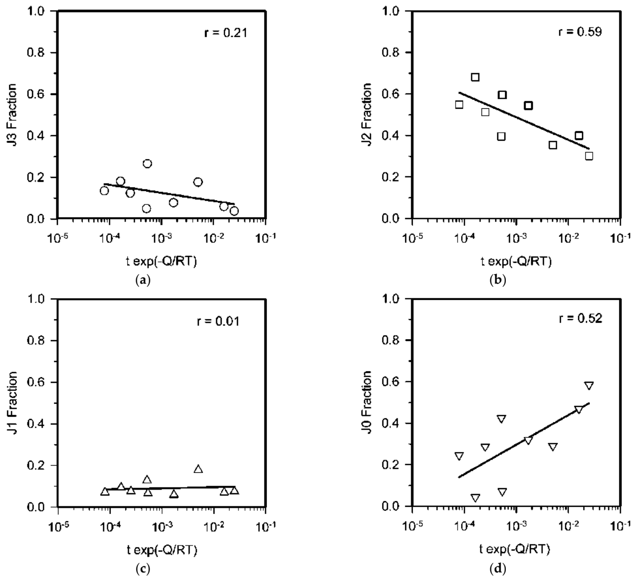
Figure 6. Effect of the temperature compensated annealing time on the fraction of triple junctions composed of three ordinary grain boundaries (a); two ordinary grain boundaries and one special boundary (b); one ordinary grain boundary and two special boundaries (c); and three special boundaries (d). The values of the determination coefficient (r) correspond to the linear regressions.
