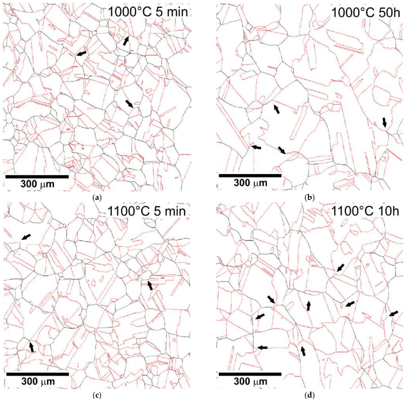
Figure 4. Grain boundary network in the steel samples annealed at 1000 °C for 5 min (a), at 1000 °C for 50 h (b), at 1100 °C for 5 min (c), and at 1100 °C for 10 h (d). Black and red lines indicate ordinary and \Sigma 3^n CSL boundaries, respectively.
