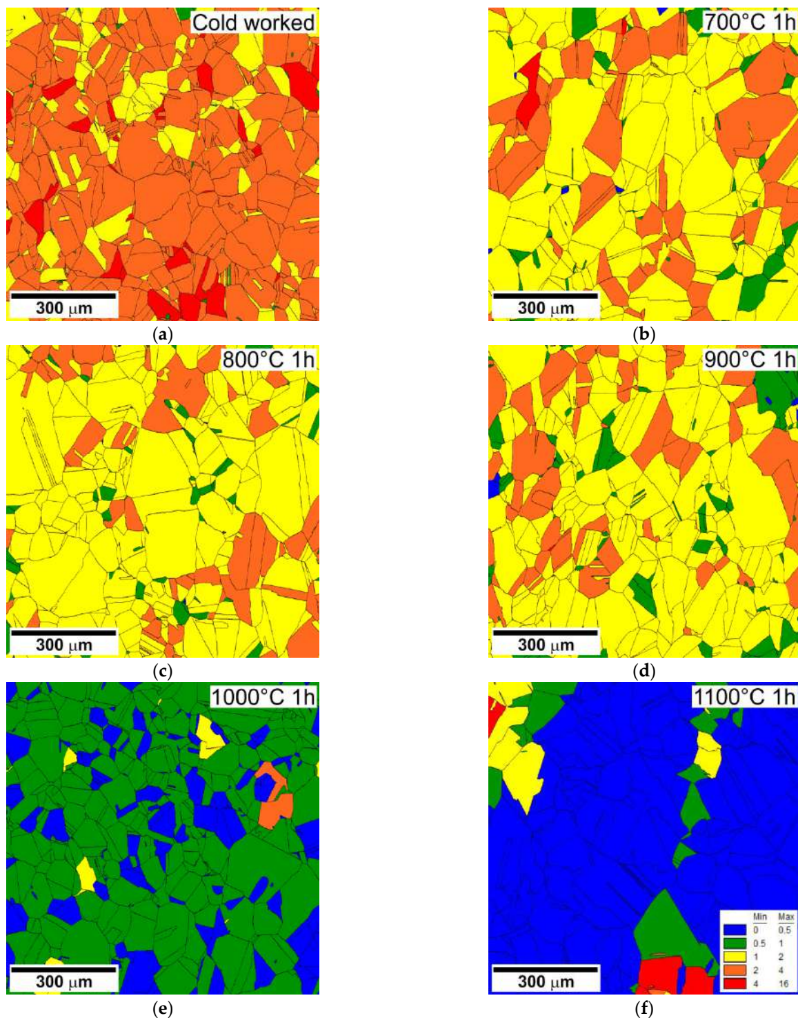
Figure 1. Grain orientation spread in the steel samples subjected to cold rolling with 5% reduction (a), and then annealed for 1 h at 700 °C (b), 800 °C (c), 900 °C (d), 1000 °C (e), and 1100 °C (f). The colour correspondence is shown in the inset in (f).
