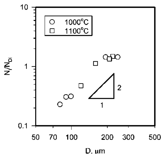
Figure 8. Relationship between the number of grain boundary interruptions per grain ( N_i/N_{Di} ) and the grain size ( D ) in a 316L stainless steel subjected to recrystallization annealing followed by grain growth.
