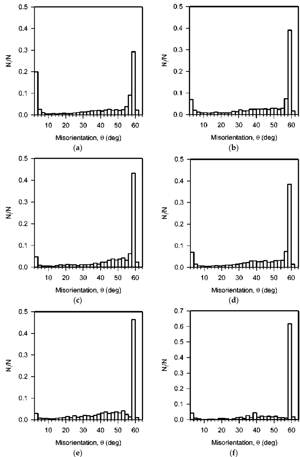
Figure 3. Grain boundary misorientation distribution in the steel samples subjected to cold rolling with 5% reduction (a), and then annealed for 1 h at 700 °C (b), 800 °C (c), 900 °C (d), 1000 °C (e), and 1100 °C (f).
