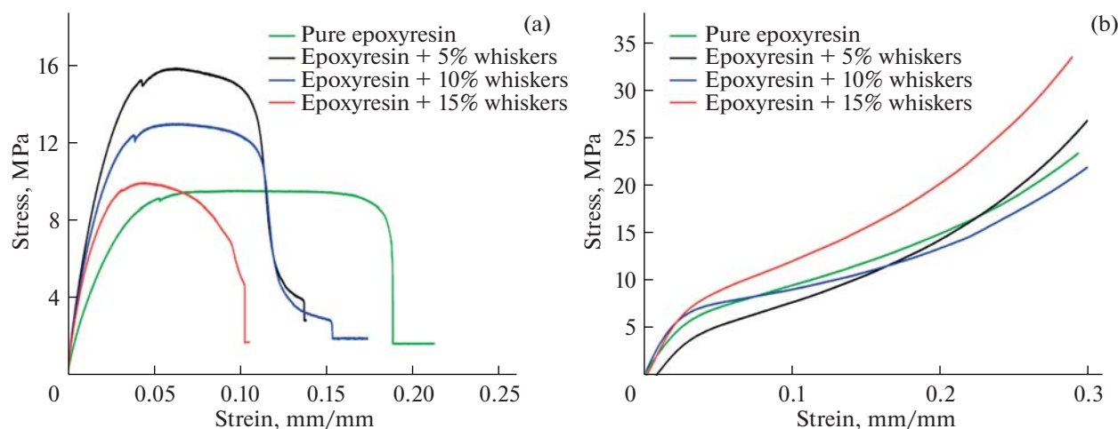
Fig. 8. (a) Stress-strain diagram for samples of composite epoxy resin containing 0, 5, 10, and 15% of \text{CaSO}_4 \cdot 2\text{H}_2\text{O} filamentary crystals, obtained in tension; (b) the same in strain compression.
