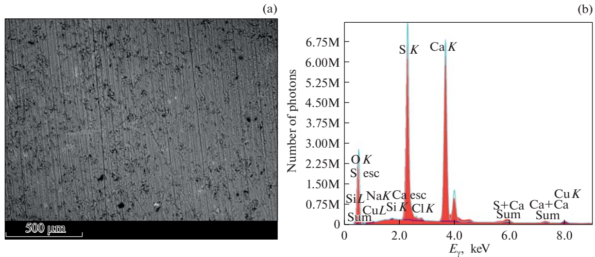
Fig. 3. SEM micrograph of the sample (\text{CaSO}_4 \cdot 2\text{H}_2\text{O})_{0.95}-(\text{CuSO}_4 \cdot 5\text{H}_2\text{O})_{0.05} slip surface using FEI Quanta 600 FEG, magnification \times 150 (a); spectrum EDX of sample (\text{CaSO}_4 \cdot 2\text{H}_2\text{O})_{0.95}-(\text{CuSO}_4 \cdot 5\text{H}_2\text{O})_{0.05} (b).
