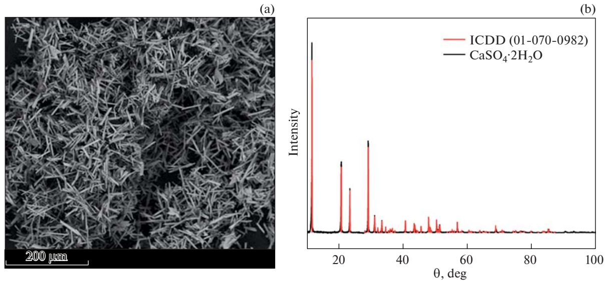
Fig. 1. SEM micrograph of \text{CaSO}_4 \cdot 2\text{H}_2\text{O} whiskers obtained on FEI Quanta 600 FEG (a), X-ray spectrum of \text{CaSO}_4 \cdot 2\text{H}_2\text{O} whiskers and test spectrum from ICDD (01-070-0982) database obtained on Rigaku SmartLab diffractometer (b).
