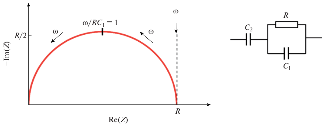
Fig. 6. Equivalent scheme of a solid-electrolyte cell with blocking electrodes without taking into account grain boundary resistance.
