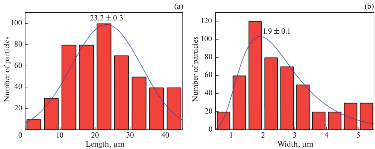
Fig. 2. Histograms of particle (whiskers) size distribution obtained from SEM images: length (a) and width (b), respectively.
