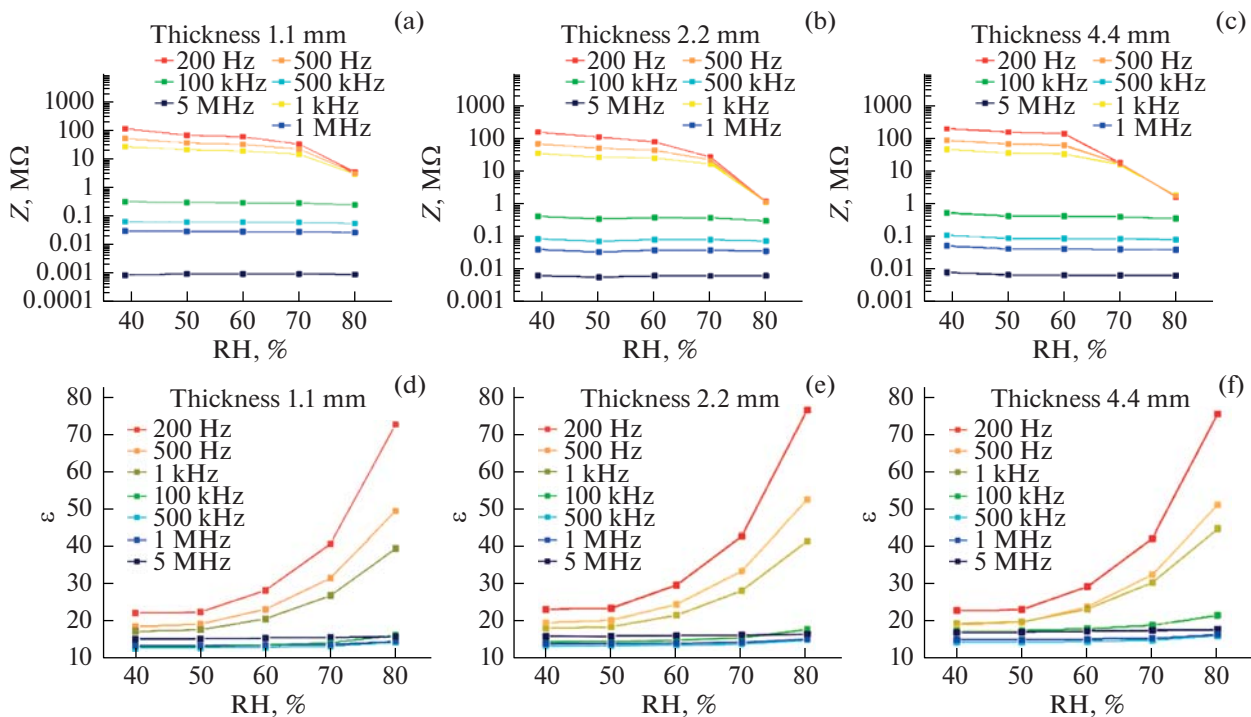
Fig. 4. Dependence of complex resistance Z on relative humidity of composite samples (\text{CaSO}_4 \cdot 2\text{H}_2\text{O})_{0.95}-(\text{CuSO}_4 \cdot 5\text{H}_2\text{O})_{0.05} of three thicknesses—1.1 (a), 2.2 (b), 4.4 mm (c). Dependence of dielectric constant \epsilon on relative humidity for samples 1.1 (d), 2.2 (e), 4.4 mm (f) with frequency variation from 200 Hz to 5 MHz.
