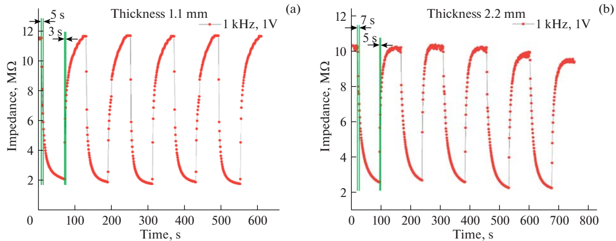
Fig. 7. Impedance switching cycles over a relative humidity range of 30–90% for samples (\text{CaSO}_4 \cdot 2\text{H}_2\text{O})_{0.95}-(\text{CuSO}_4 \cdot 5\text{H}_2\text{O})_{0.05} thicknesses of 1.1 (a) and 2.2 mm (b).
