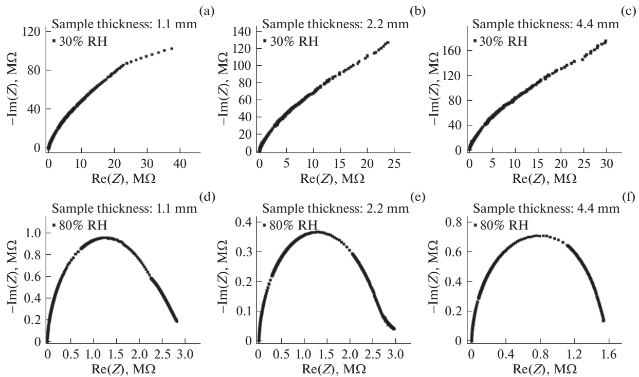
Fig. 5. Impedance spectroscopy results of samples (\text{CaSO}_4 \cdot 0.5\text{H}_2\text{O})_{0.95}-(\text{CuSO}_4 \cdot 5\text{H}_2\text{O})_{0.05} of three thicknesses—1.1, 2.2, and 4.4 mm at a relative humidity range of 30–80%.
