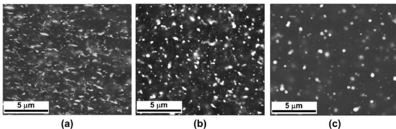
Figure 4. Typical backscatter electron images of the precipitates acquired from the central section of the stir zone of the low-heat-input weld (a) in the as-welded condition, (b) after heating to 450 °C, and (c) after heating to 500 °C.
