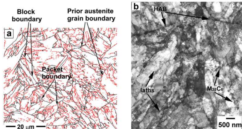
Figure 1. Typical hierarchical microstructure in 9–12% Cr steels on the example of boundary map of the as-tempered 10Cr steel (black and red lines correspond to high-angle and low-angle boundaries, with misorientations of \theta \geq 15^\circ and 2^\circ \leq \theta < 15^\circ , respectively), showing the prior austenite grains divided on blocks and packets with martensite laths (a). TEM micrograph showing the laths structure with high dislocation density and precipitated M_{23}C_6 carbides on the lath boundaries and high-angle boundaries (HABs) (b). Reprinted with permission from Ref. [8]. Copyright 2019 Elsevier.
