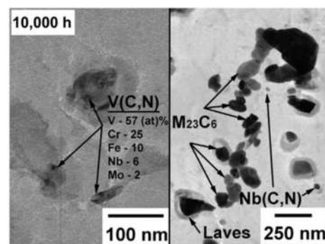
Figure 25. TEM micrograph (extraction replica) showing the precipitated fine V-rich M(C,N) particles at the apparent steady-state creep stage (10,000 h) in the 10Cr steel. Reprinted with permission from Ref. [15]. Copyright Elsevier 2018.
