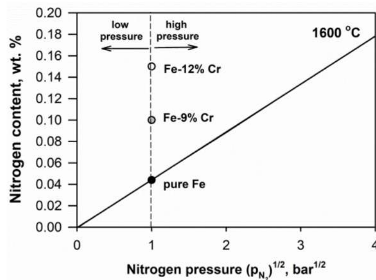
Figure 2. Effect of nitrogen partial pressure on nitrogen solubility in liquid pure Fe at 1600 °C. Points for Fe–Cr alloys show the effect of Cr content on the nitrogen solubility. Data from [60].
