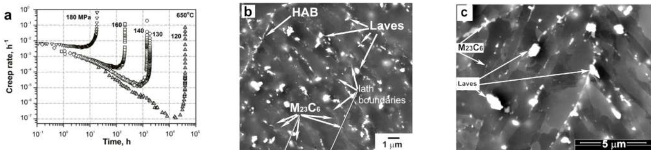
Figure 16. Creep rate vs. time curves of the 10Cr steel at 650^\circ\text{C} and different applied stresses from 120 to 180 MPa (a). The lath structure and dispersion of particles in the 10 Cr steel at the apparent steady-state creep stage at 650^\circ\text{C} and 120 MPa, 10,000 h on the high-angle boundary (HAB) and lath boundaries (b) Reprinted with permission from Ref. [8], Copyright Elsevier 2019; after creep rupture test for 39,437 h (c). Reprinted with permission from Ref. [15], Copyright Elsevier 2018.
