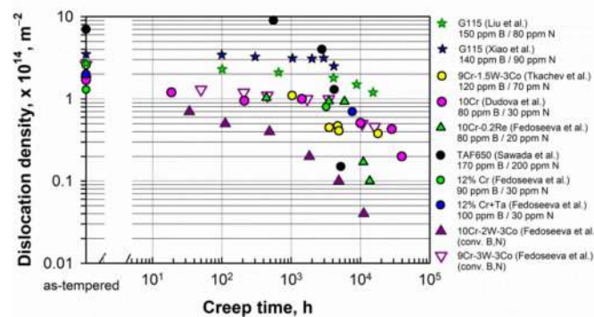
Figure 20. Evolution of the dislocation density during creep in the 9–12% Cr steels. Data from [8,16,17,21,22,38,39,49,71].
