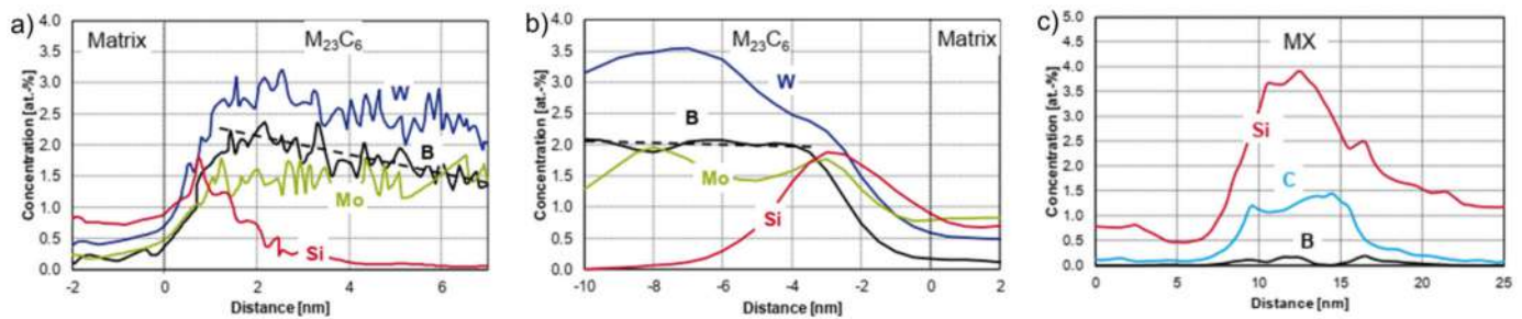
Figure 18. Proxigram analysis showing quantitative B, W, Mo, Si concentration profiles across M_{23}C_6 /matrix (a,b) and B, C, and Si concentration profiles across MX/matrix (c) interface in the SuperVM12 steel after creep at 650 °C for 23,844 h. Reprinted with permission from Ref. [54]. Copyright 2019 ASM International.
