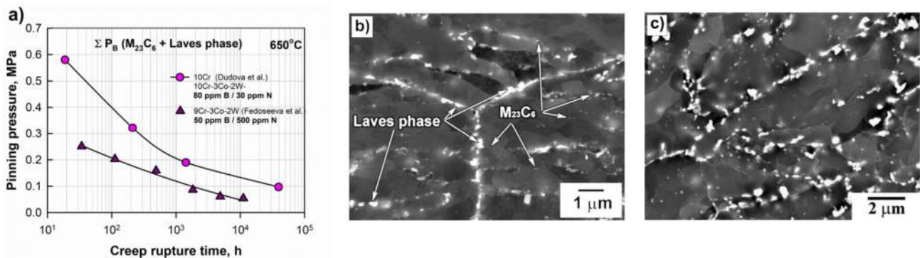
Figure 26. Change in the pinning pressure from M_{23}C_6 carbides and Laves phase particles on the grain and lath boundaries of the 10Cr steel with increased B and decreased N contents and the 9Cr-3Co-2W steel with conventional B and N contents during creep tests at 650 °C and different applied stresses 180–120 MPa (a). Data from [8,21]. Microstructure of the steels after creep tests at 650 °C under a stress of 140 MPa: (b) the 10Cr steel, 1426 h, reprinted with permission from Ref. [82], Copyright 2016 Elsevier; (c) the 9Cr-3Co-2W steel, 1828 h, reprinted with permission from Ref. [21], Copyright 2016 Elsevier.
