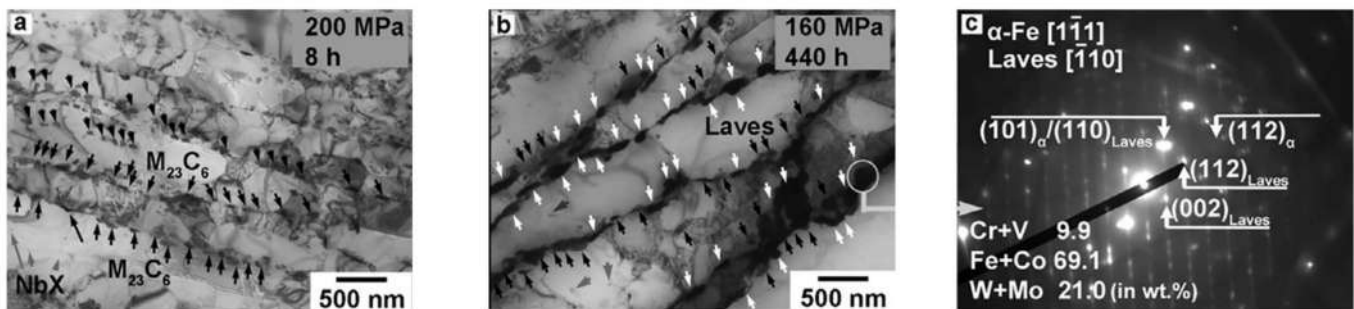
Figure 17. TEM micrographs of the 10Cr-0.2Re steel after short-term creep tests at 650 °C: 200 MPa, 8 h (a) and 160 MPa, 440 h (b); black and white arrows indicate M_{23}C_6 and Laves phase particles, respectively, located along the lath boundaries; grey arrows indicate NbX particles precipitated within the laths. Electron diffraction pattern (c) is obtained from the Laves phase particle shown by circle in (b). Reprinted with permission from Ref. [74], Copyright Elsevier 2018.
