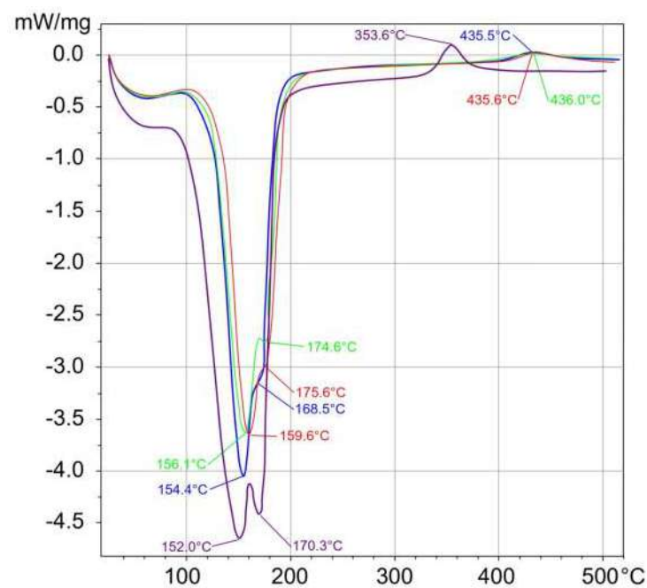
Figure 2. DTA-diagrams of PGs and NG. — NG; — \text{PG}_{\text{Bel}} ; — \text{PG}_{\text{Bal}} ; — \text{PG}_{\text{Kin}} .
