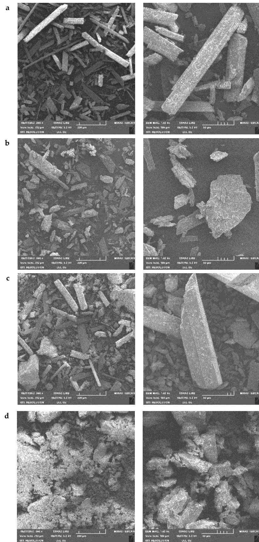
Figure 8. Morphology of the binder based on: (a)—PG Bel ; (b)—PG Bal ; (c)—PG Kin ; (d)—NG.
