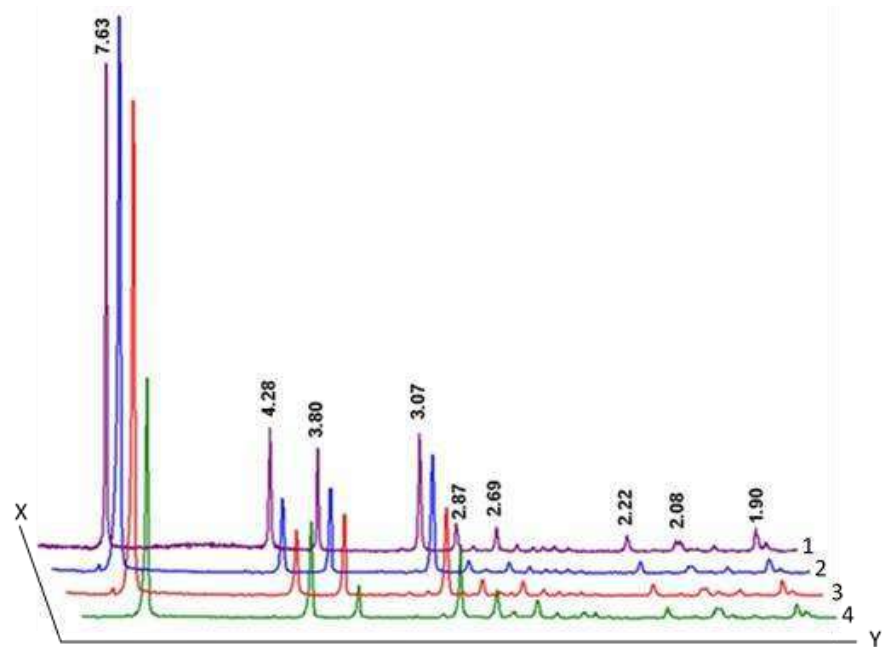
Figure 1. XRD-diagram of PGs and NG. — NG (1); — \text{PG}_{\text{Bel}} (2); — \text{PG}_{\text{Bal}} (3); — \text{PG}_{\text{Kin}} (4).
