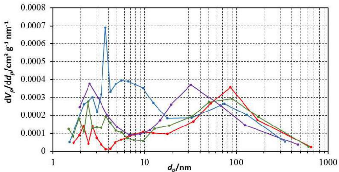
Figure 9. Pore volume distribution for binders, based on: — NG ; — PG_{Bel} ; — PG_{Bal} ; — PG_{Kin} .
