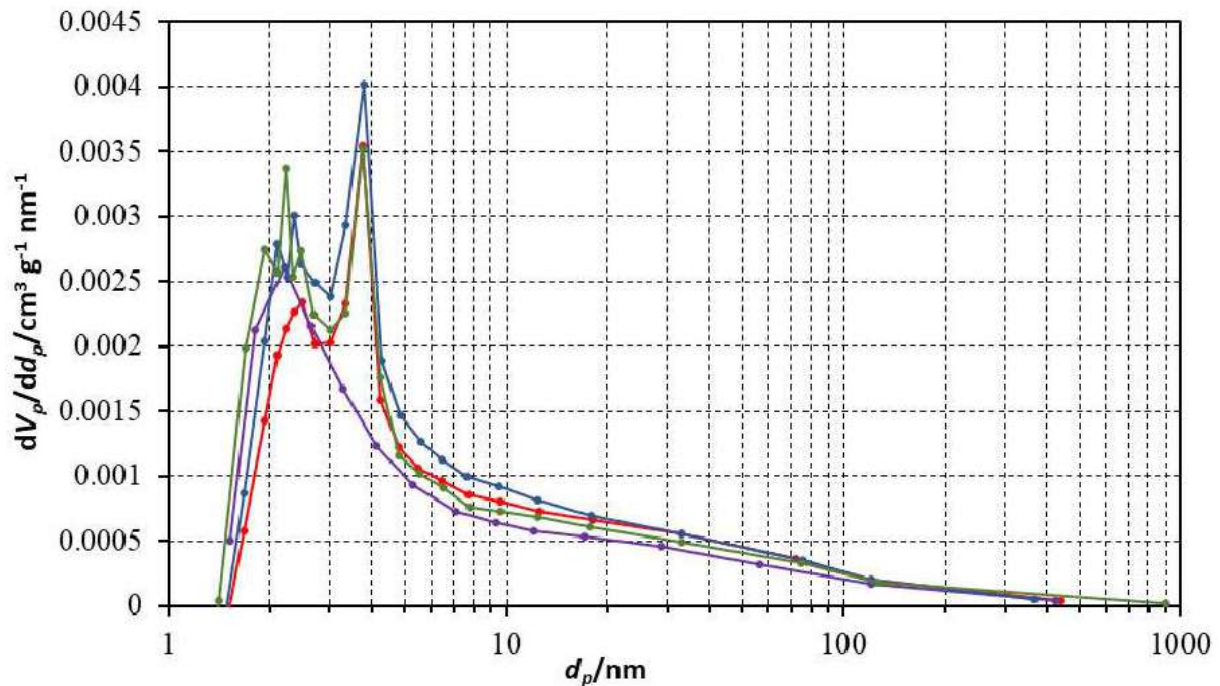
Figure 7. Pore size distribution of PGs and NG. — NaG; — PG Bel ; — PG Bal ; — PG Kin .
