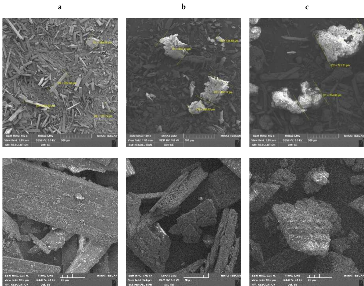
Figure 3. Morphology of the PGs particles. (a)— PG_{Bel} ; (b)— PG_{Bal} ; (c)— PG_{Kin} .
