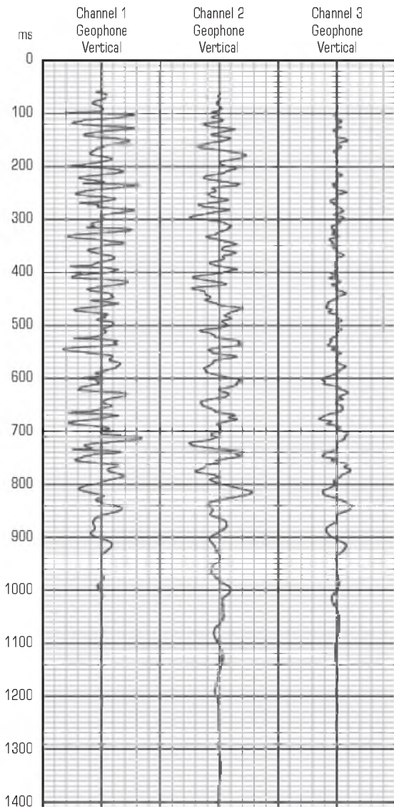
Fig. 3. Representative seismogram from geophone on soil–cement pile top during blast no. 81: v_2 (R) = 5.71 \text{ mm/s} ; R = 26 \text{ m}
