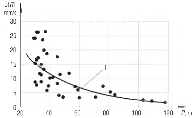
Fig. 4. Function v (R) versus distance R at caisson bottom: • – experiment; 1 – theoretical curve from (3)
