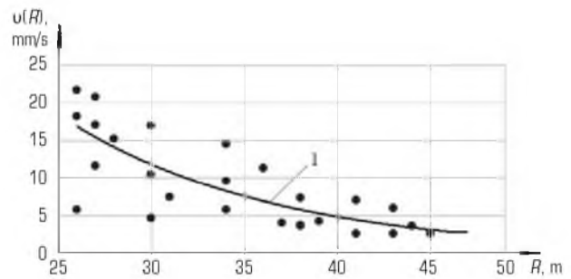
Fig. 5. Function v (R) versus distance R at soil–cement pile top: • – experiment; 1 – theoretical curve from (4)
