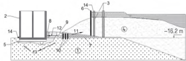
Fig. 1. Layout of gneissic granite rock mass (1), caisson (2), soil–cement piles (3) and blasting site; 4 – sand and sand clay; 5 – caisson foundation bed; 6 – metallic retention wall; 7 – gneissic granite rock mass to be treated; 8 – cushioning bags filled with expanded-clay aggregate; 9 – blasted rocks; 10 – blastholes; 11, 12 and 13 – directions of blasting-induced seismic waves; 14 – locations of geophones
