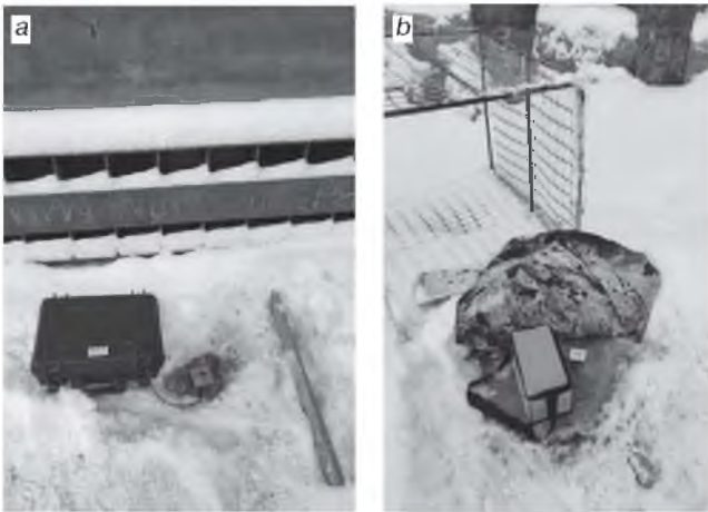
Fig. 2. a – Geophone arranged on caisson foundation bed (large-scale blast no. 81 on Dec 3, 2021); b – geophone arranged atop of soil–cement pile (large-scale blast no. 81 on Dec 3, 2021)
