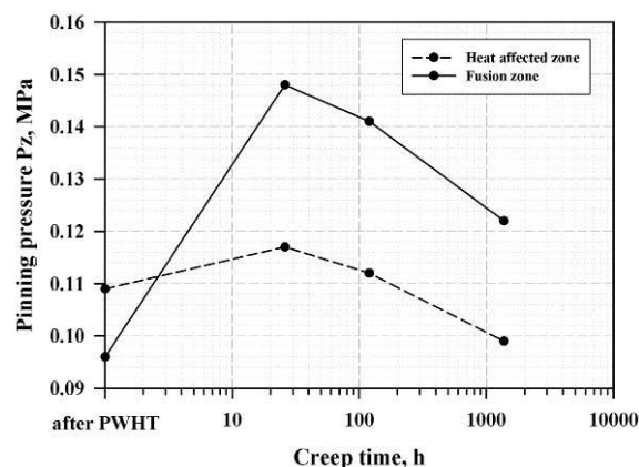
Figure 3. The evolution of Zener pinning pressures exerted by precipitates in HAZ and FZ of the studied weld joint during creep exposure.
