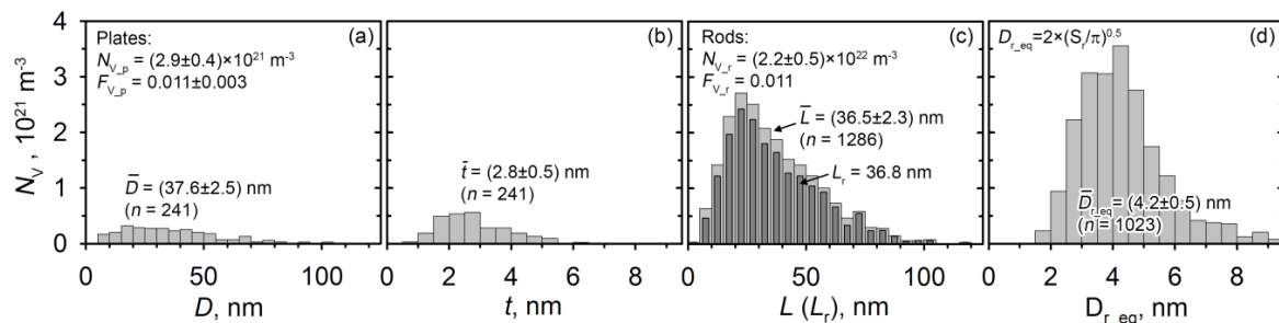
Figure 2. The plate diameter (a) and thickness (b) as well as true rod length (c) and equivalent circular diameter (d) distributions in the aged at 170°C for 96 h. N_{V,p} , N_{V,r} , \bar{D} , \bar{t} , \bar{L} (‘rectangle’ length in \{100\}_{\text{Al}} projection), \bar{D}_{r,eq} and F_{V,p} (for the plates) were averaged using at least three TEM images in respective projections.
