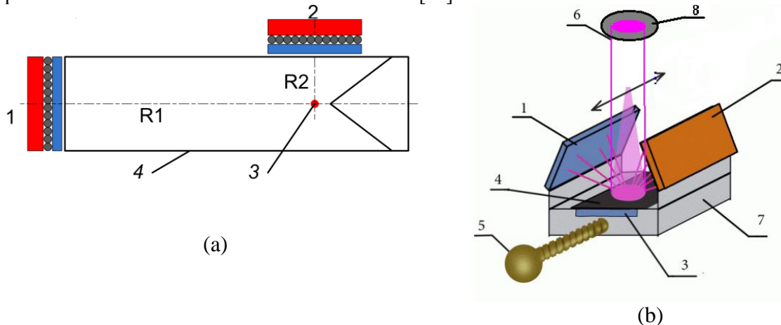
Figure 1. (a) The layout of the He-3 detector on the HELIS installation. 1 and 2 - two positions of the {}^3\text{He} detector ( R_1 = 120 cm, R_2 = 30 cm), 3 - the location of the target, 4 - contours of the HELIS installation. (b) The layout of the target and track detectors in the ion beam in the HELIS setup. 1, 2, 3 - track detectors CR-39 with different coatings; 4 - target; 5 - the manipulator; 6 - ion beam; 7 - steel substrate; 8 - diaphragm.
