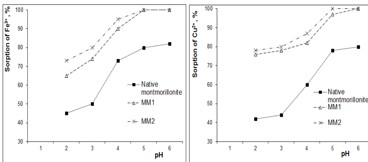
Figure 3: Effect of pH-factor on the sorption of metal ions (at initial concentration of metal ions = 0,1 mmol/l and temperature = 25 °C)
