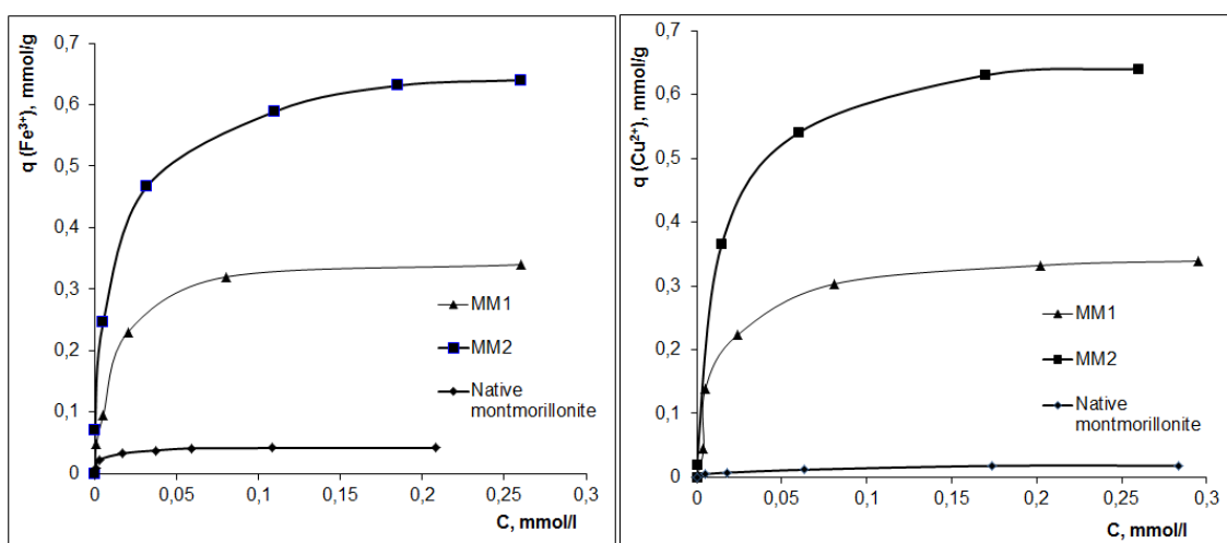
Figure 4: Sorption isotherm of \text{Fe}^{3+} and \text{Cu}^{2+} ion on native and modified forms of montmorillonite as a function of equilibrium metal ion concentration at pH 4.5 and temperature 25^\circ\text{C}
