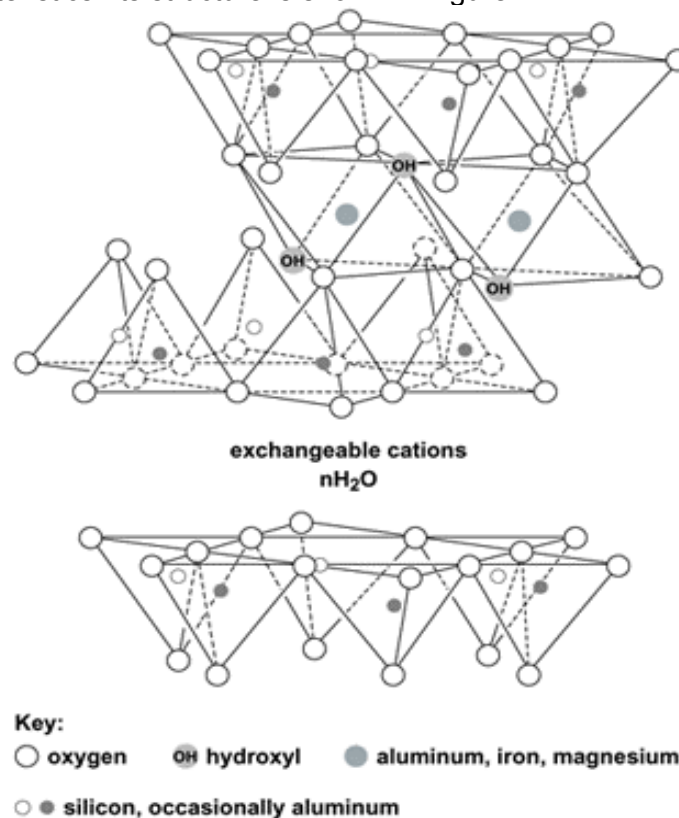
Figure 1: Structure of montmorillonite (Grim, 1953)
