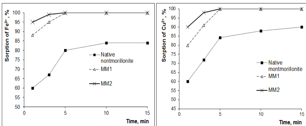
Figure 2: Effect of contact time on the sorption of metal ions (at initial concentration of metal ions = 0,1 mmol/l and temperature = 25 °C)
