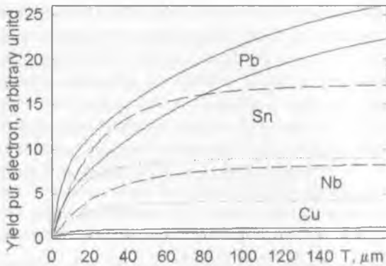
Fig. 3. The dependence of the detector response from the emission spectra hitting on the target, its material and thickness.
