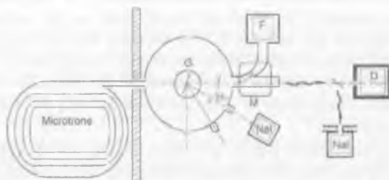
Fig. 1. Experimental setup
