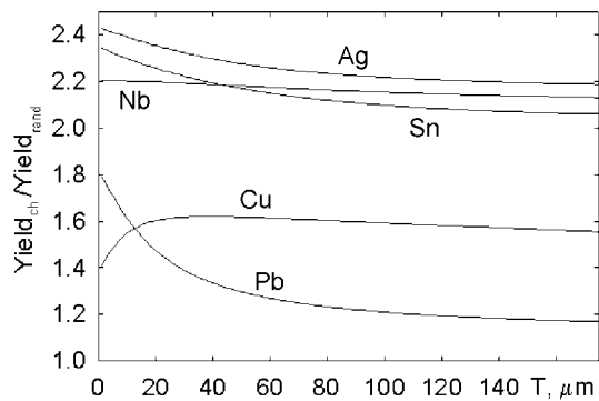
Fig.4. The dependence of the detector response correlation for emission with different thickness from the target material and thickness
