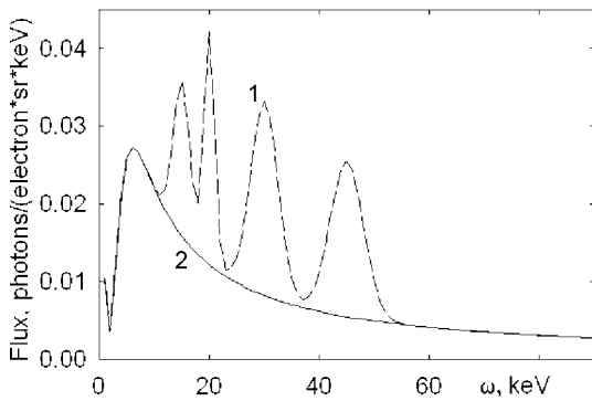
Fig.2. The emission spectra of electrons energy of 30\text{ MeV} in the silicon crystal thickness of 15\text{ }\mu\text{m} for the condition of Ref.[15]
